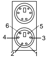
PS/2 Keyboard
